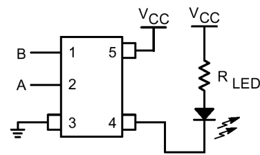
Figure 8. LED Driver
